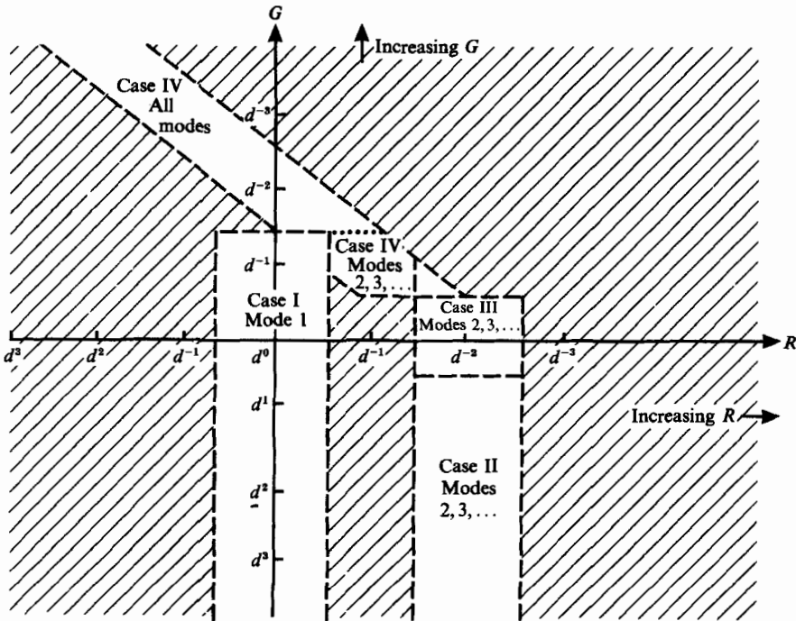
FIGURE 1. Regions of (\log_4 R, \log_4 G) -space covered by solutions near the neutral curves in the four cases of §4.1, for the shallow layer d \ll 1 , and for small wavenumbers \tilde{k} = k/d = O(1) .
